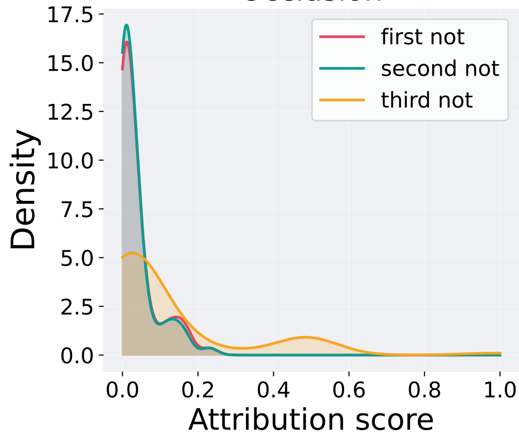
Occlusion
