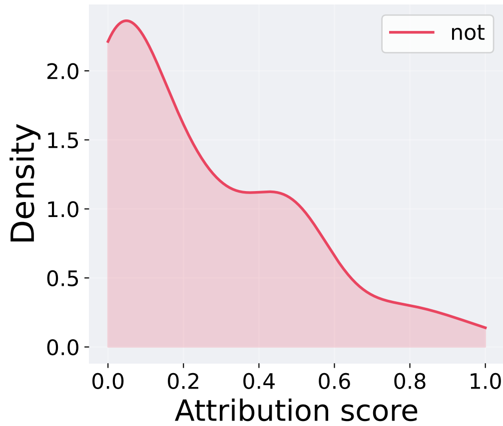
Occlusion
