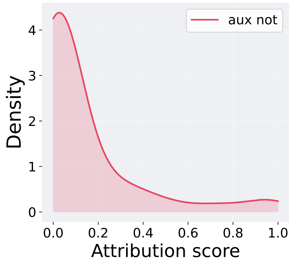
Occlusion
