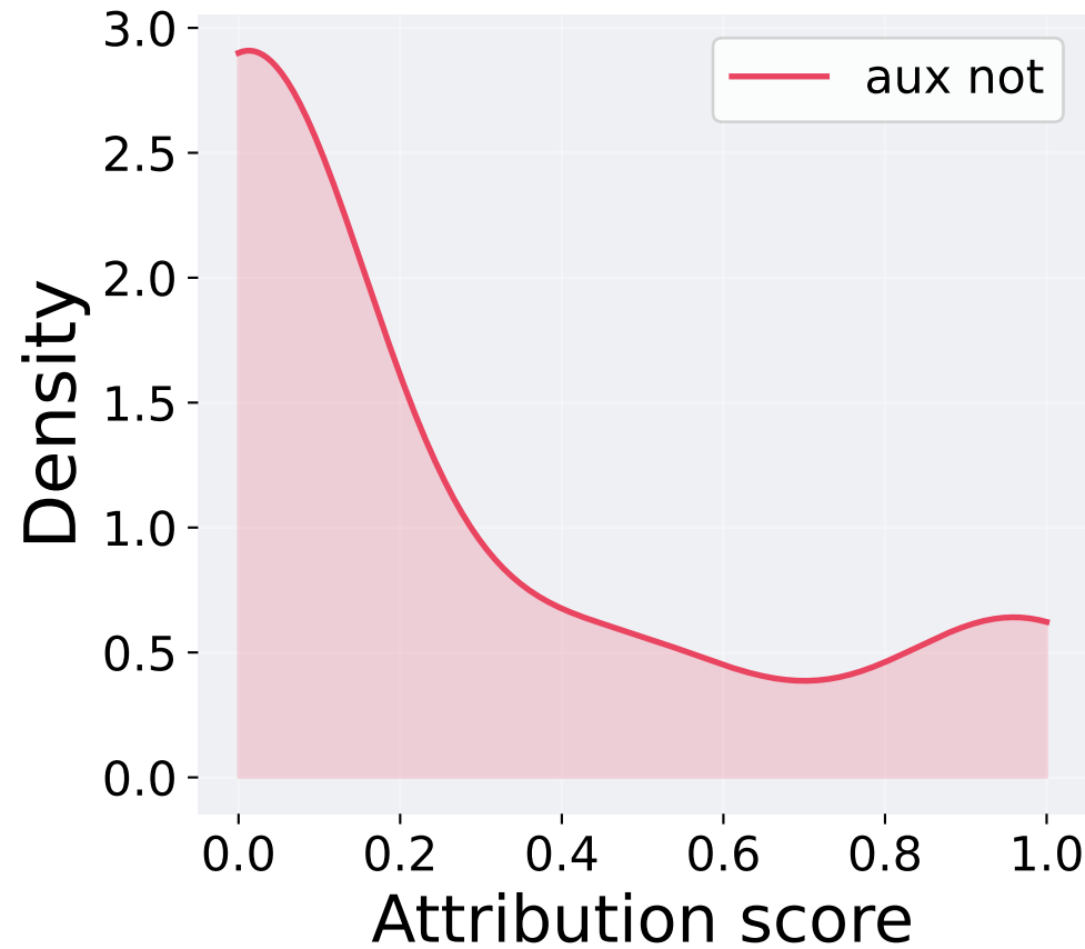
Occlusion
