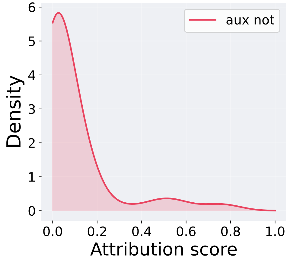
Occlusion
