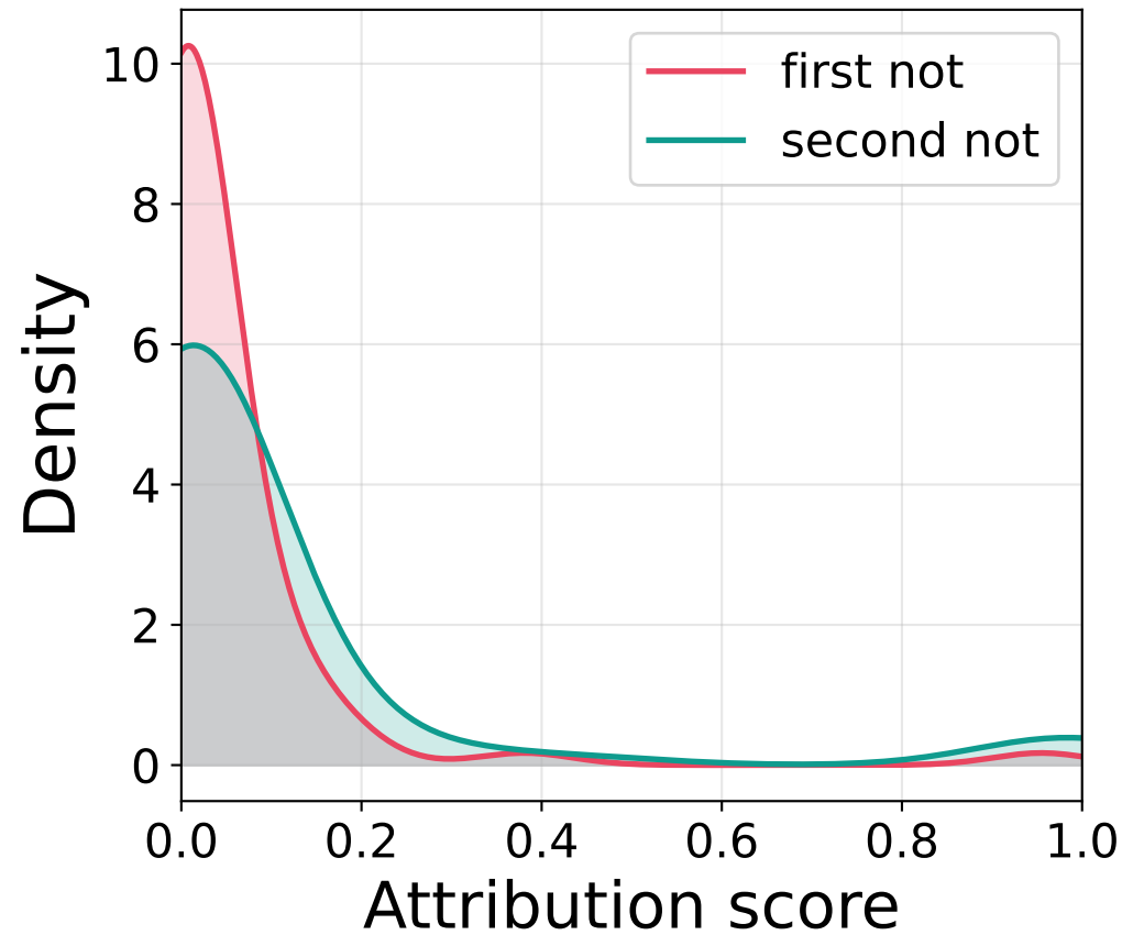
Occlusion
