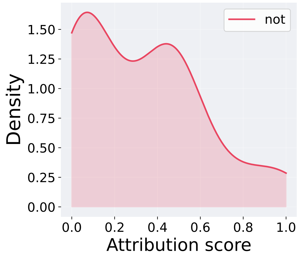
Occlusion
