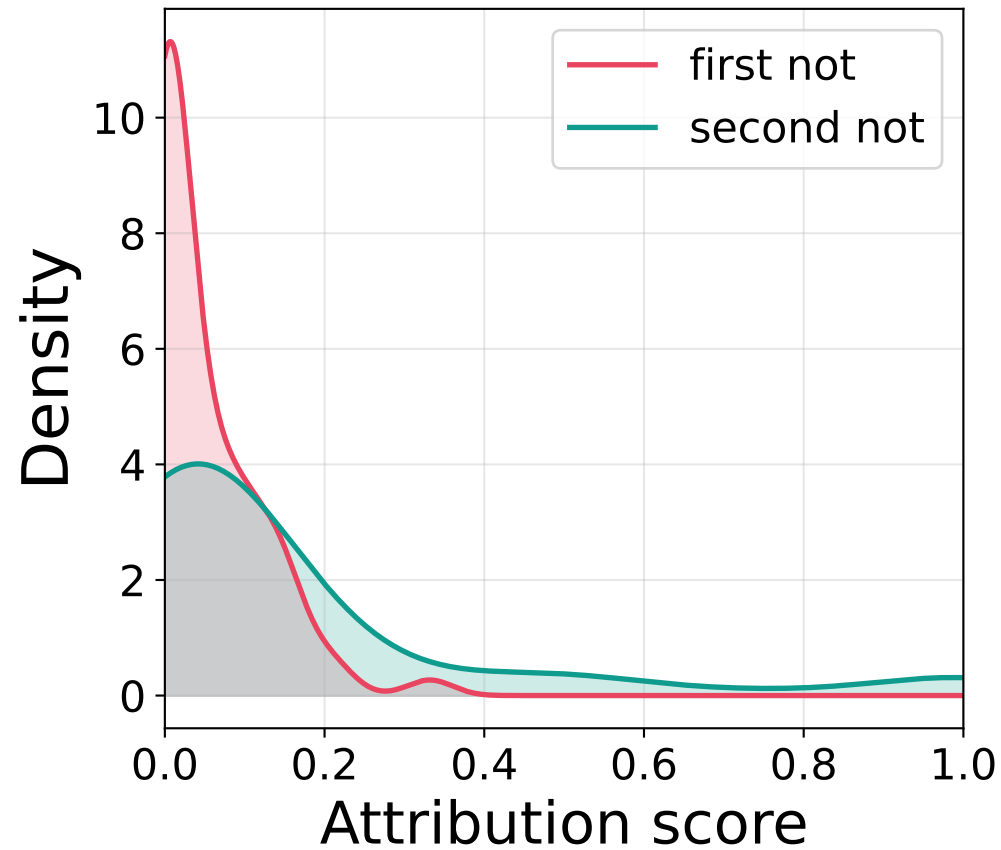
Occlusion
