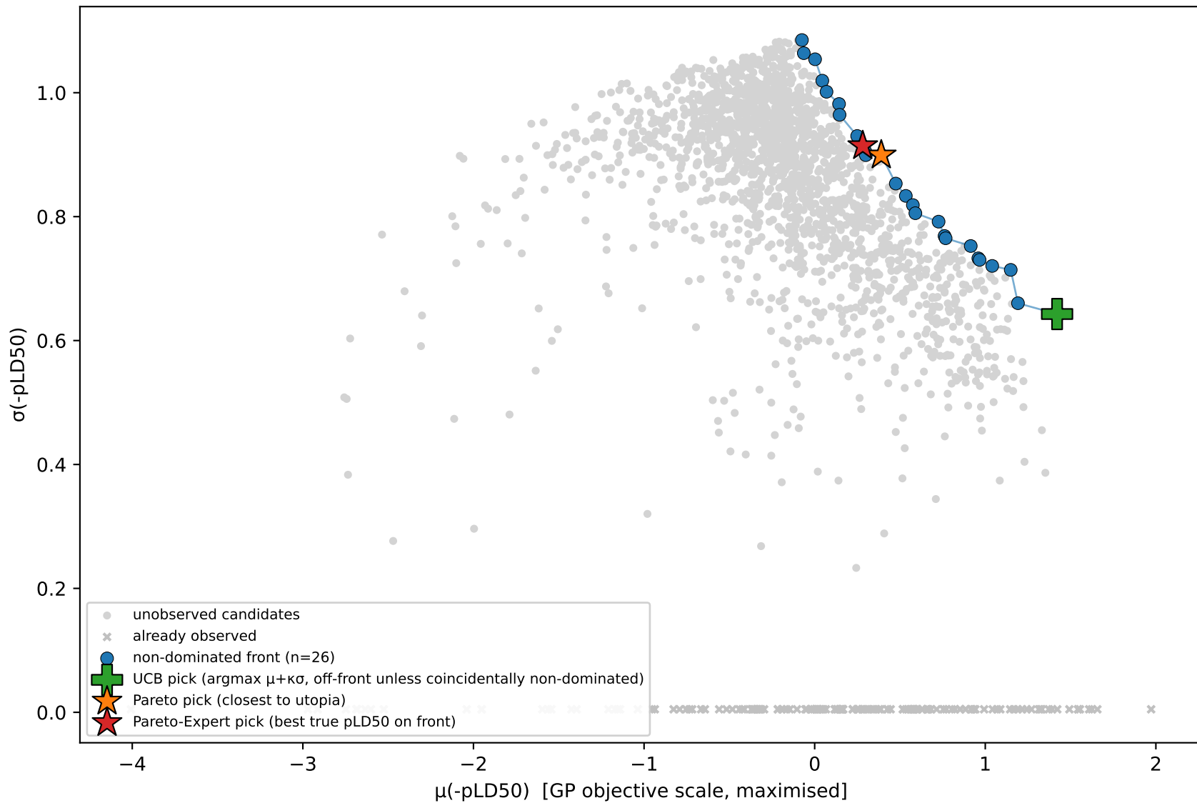
Real Pareto front, seed 11, iteration 50 (150 molecules observed so far; real VAE checkpoint + candidate pool)
