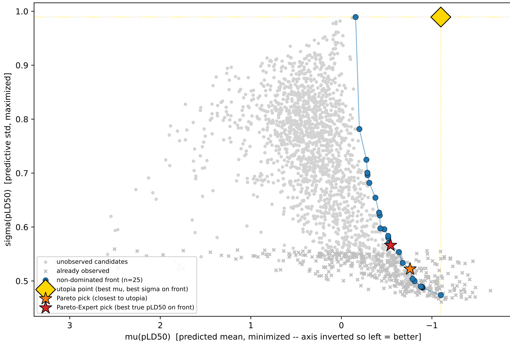
Real Pareto front, seed 11, iteration 300 (400 molecules observed so far; real VAE checkpoint + candidate pool)
