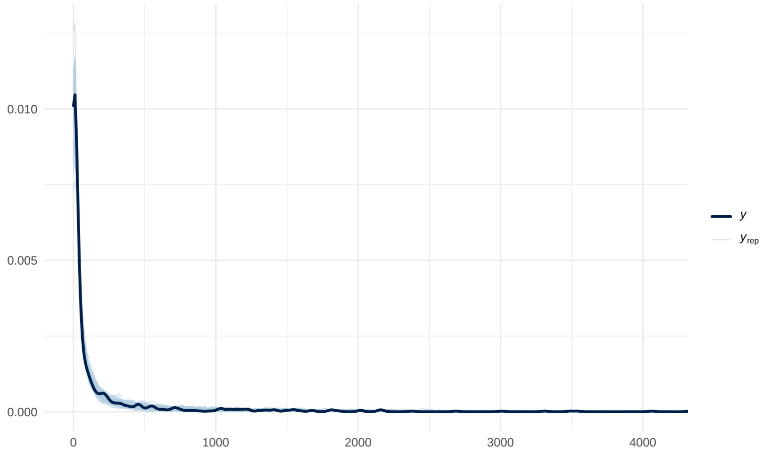
PPC: count distribution (observed vs 100 posterior draws)
