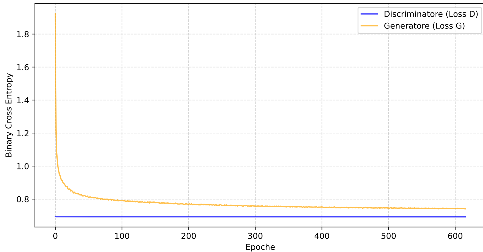
QST-CGAN Losses
