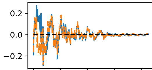
population correlation
