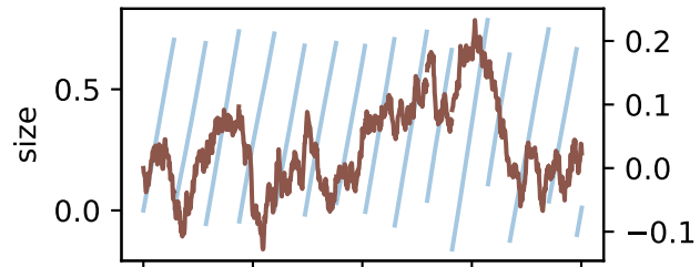
lineage dynamics
