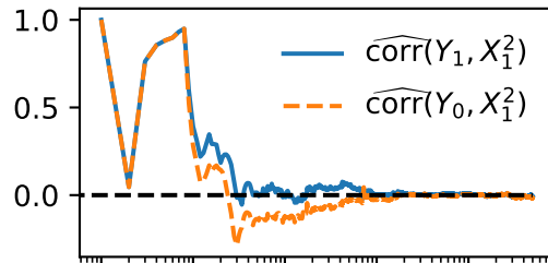
lineage correlation
