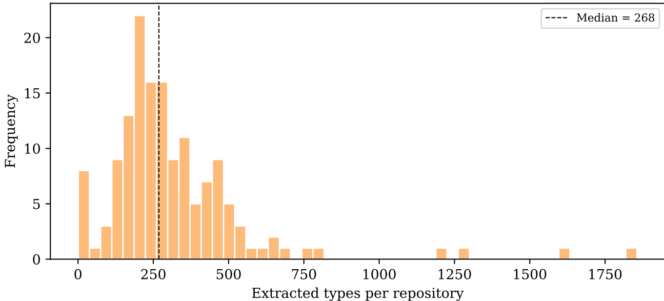
C++ Type Extraction (n=148 repos)
