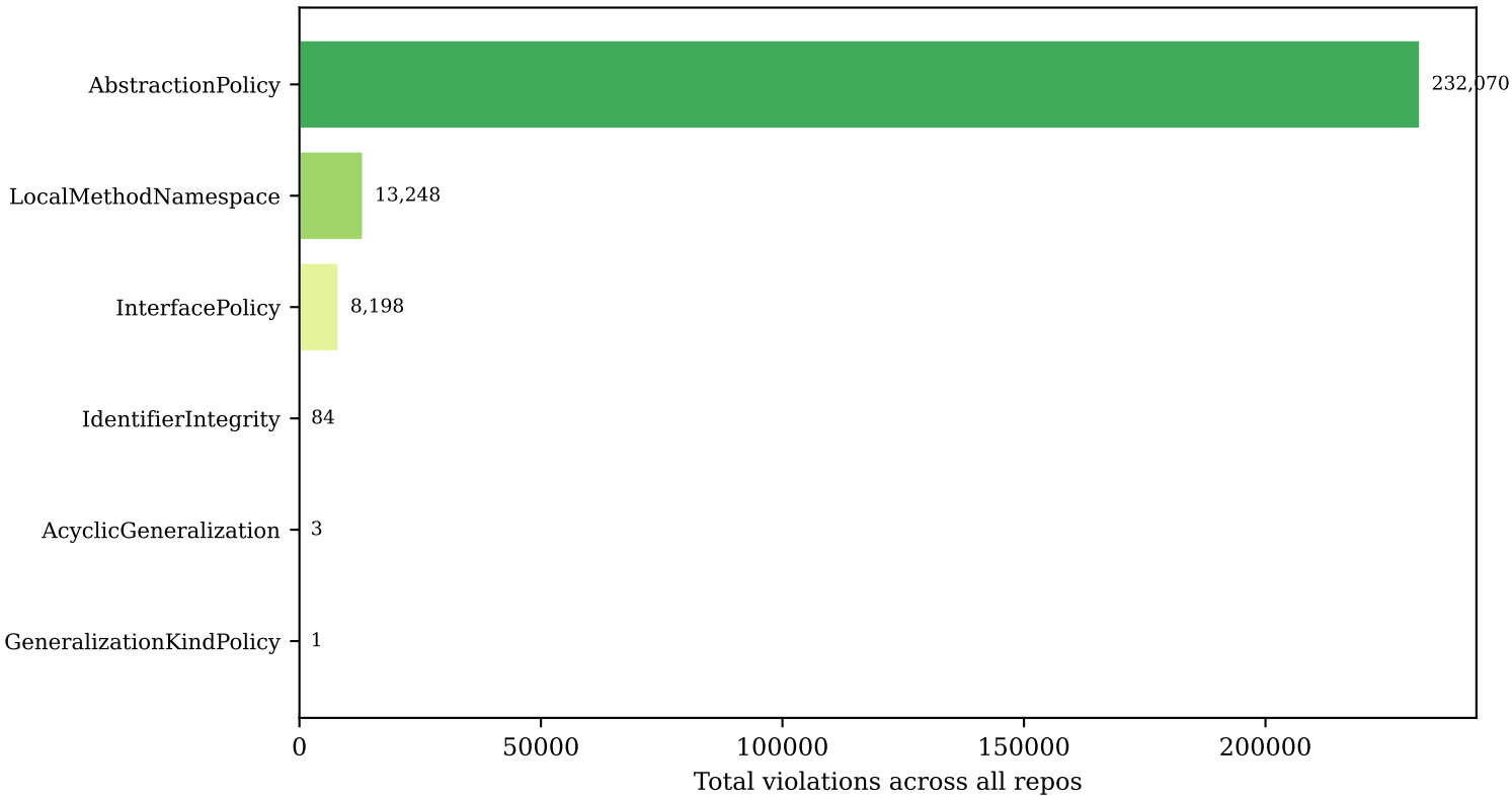
Violation Count by Invariant (Java, n=558 repos)
