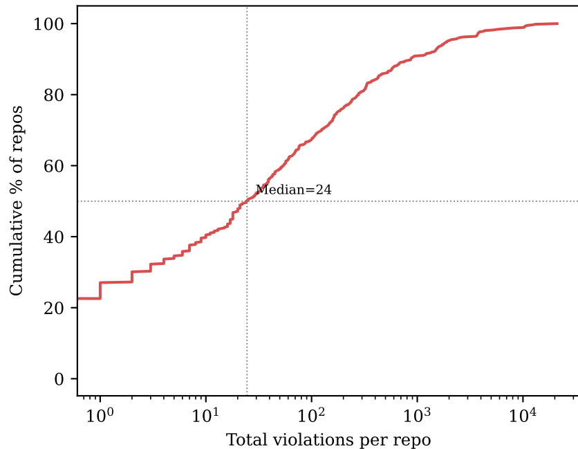
Cumulative violation distribution
