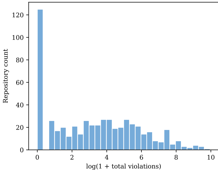
Repo-level violation intensity
