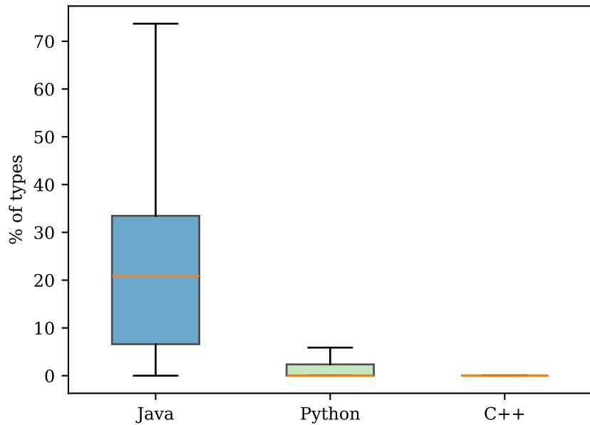
Types with interfaces
