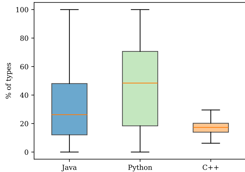
Types with superClass
