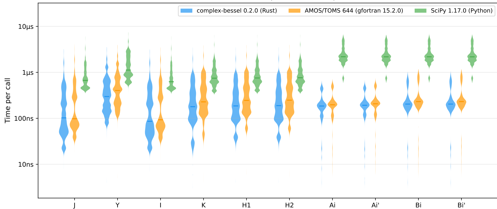
Evaluation Time (lower is better)
