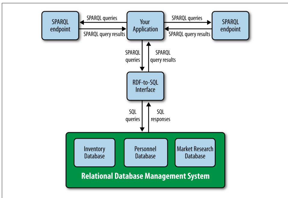
Figure 10-4. Relational database SPARQL endpoint middleware lets your application communicate with relational databases as if they were SPARQL endpoints
