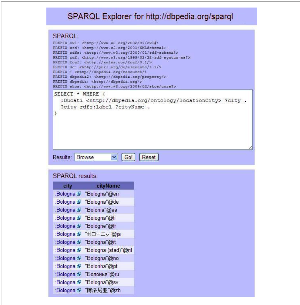
Figure 5-1. Using SNORQL to query DBpedia for Ducati's location
