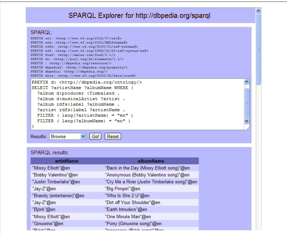
Figure 3-2. Albums produced by Timbaland, restricted to English-language data
