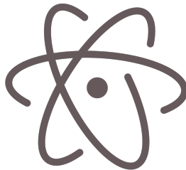
FIGURE 4.9 – Logo ATOM
