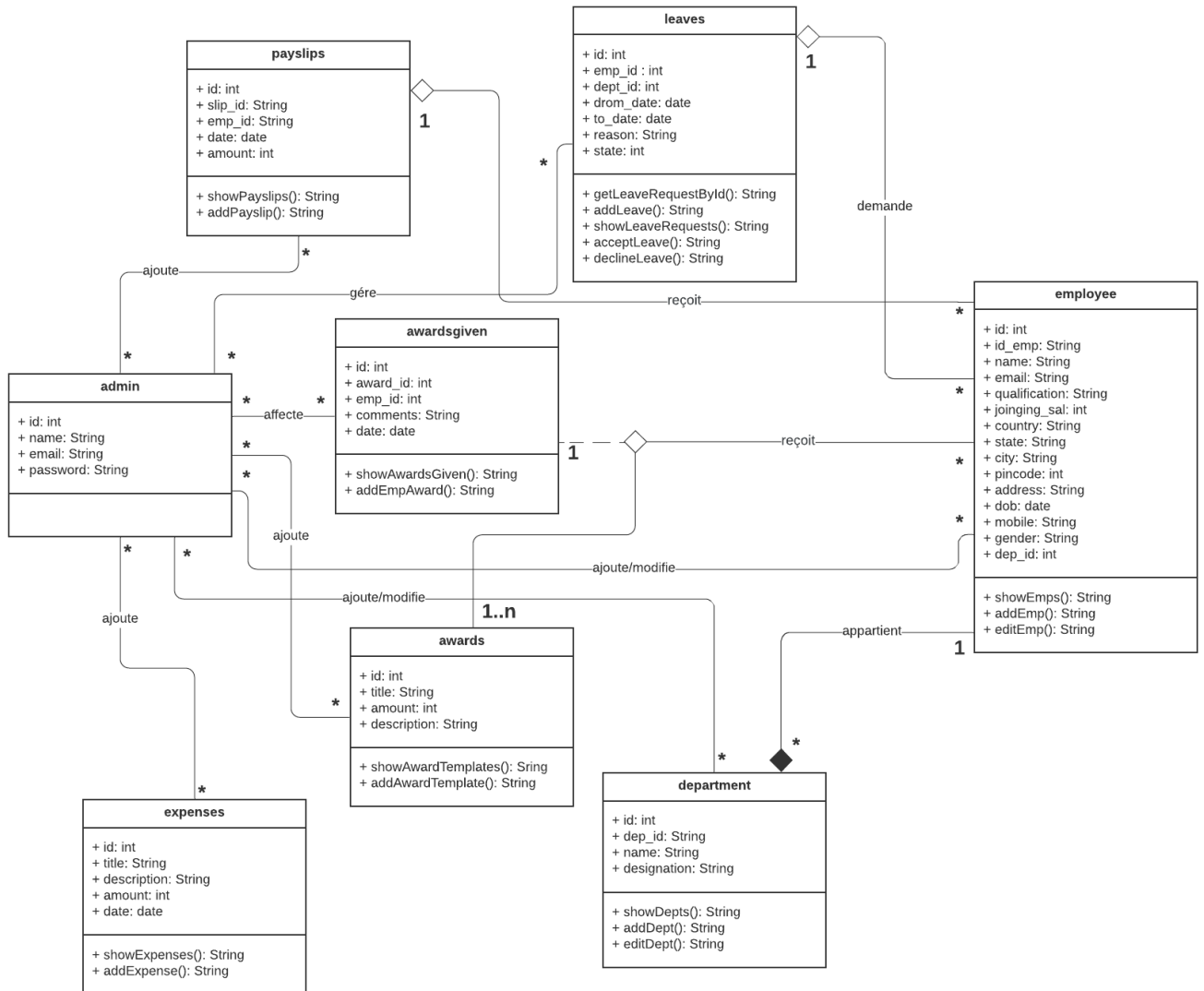
FIGURE 3.4 – Diagramme de classes
