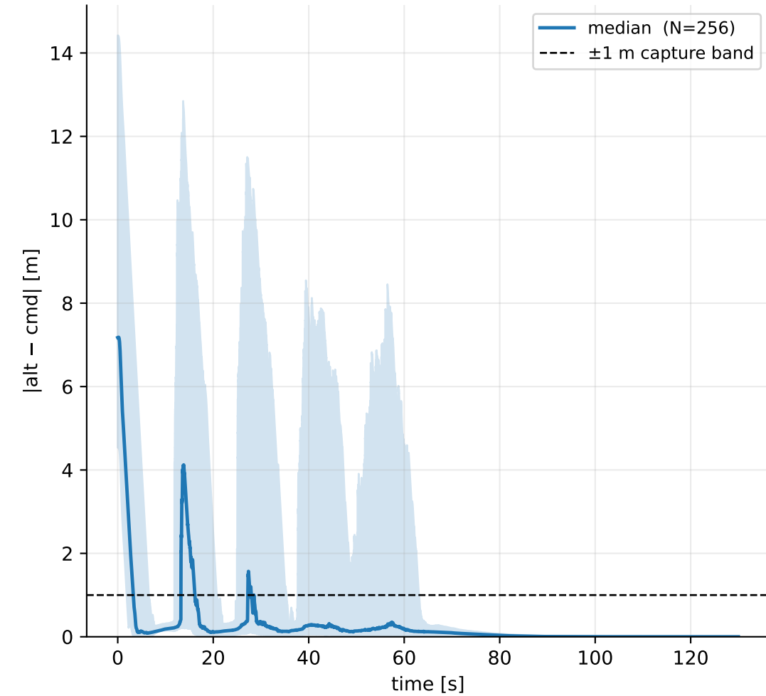
tracking error — 256 Monte Carlo episodes (10-90% band)
