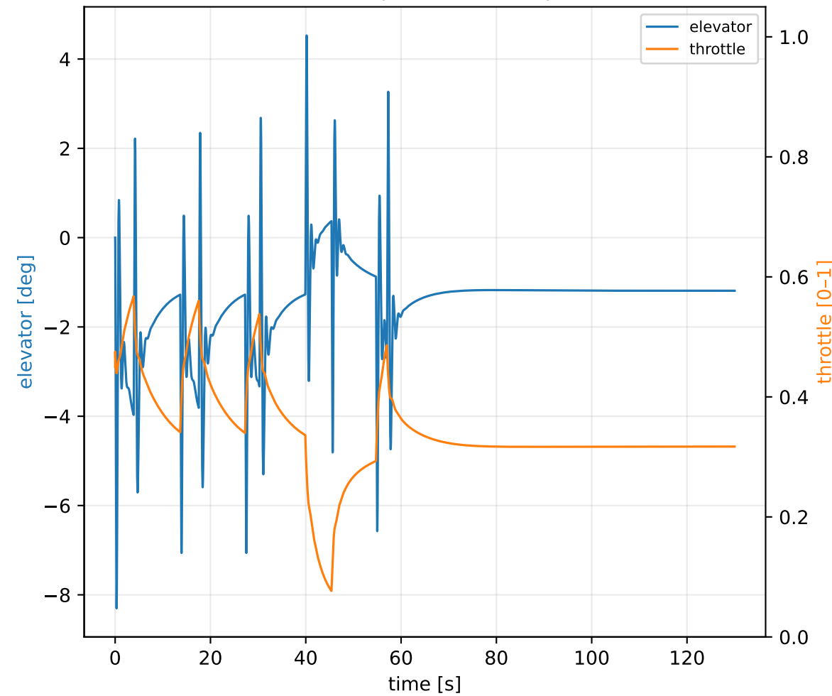
controls — representative episode
