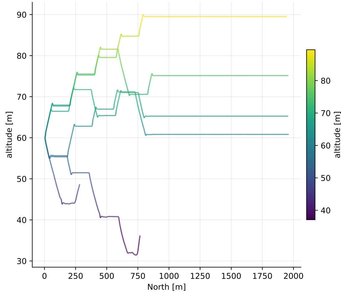
side view (colour = altitude [m])
