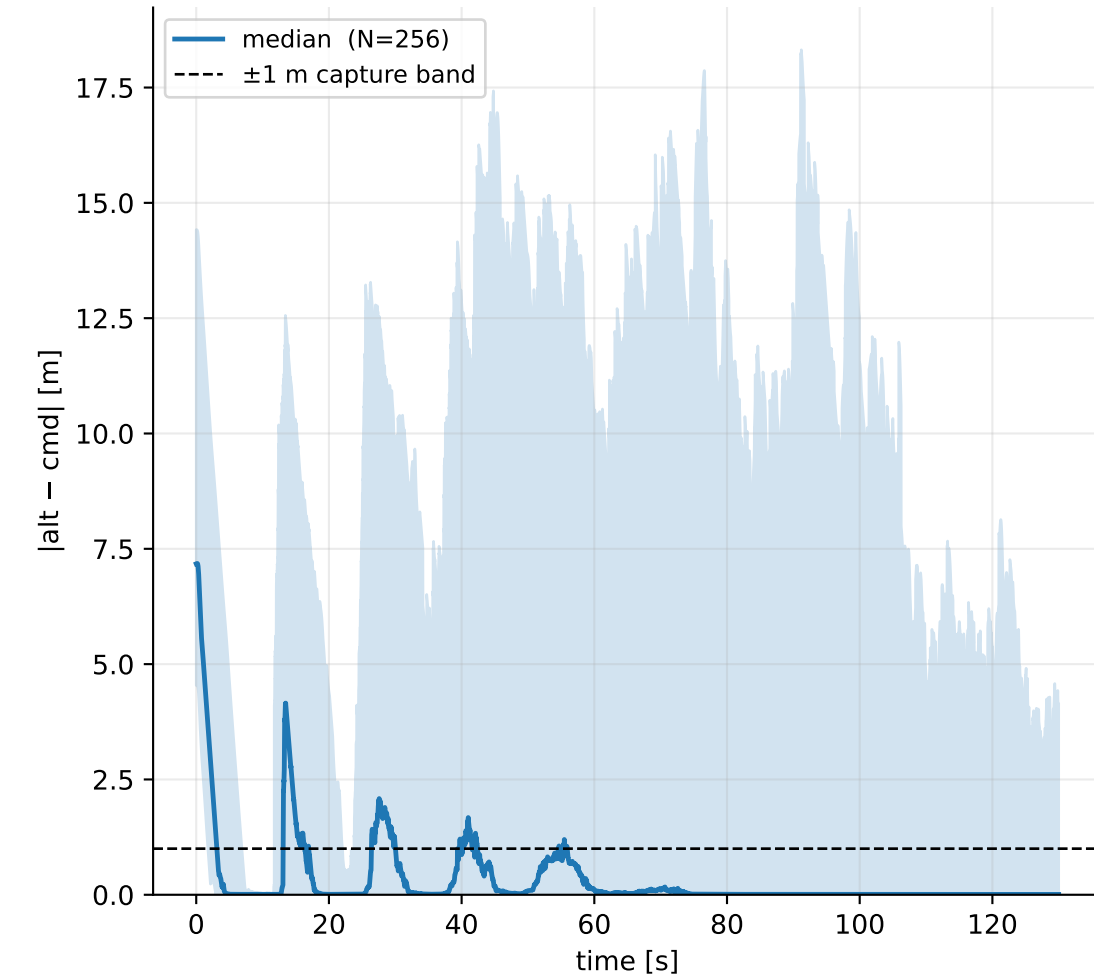
tracking error — 256 Monte Carlo episodes (10-90% band)
