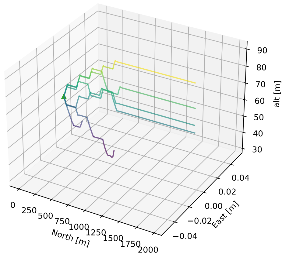
3D flight paths (colour = altitude [m])
