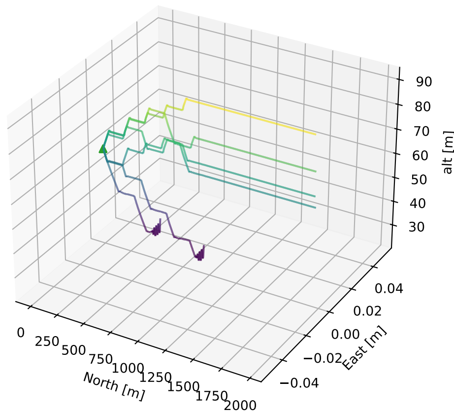
3D flight paths (colour = altitude [m])
