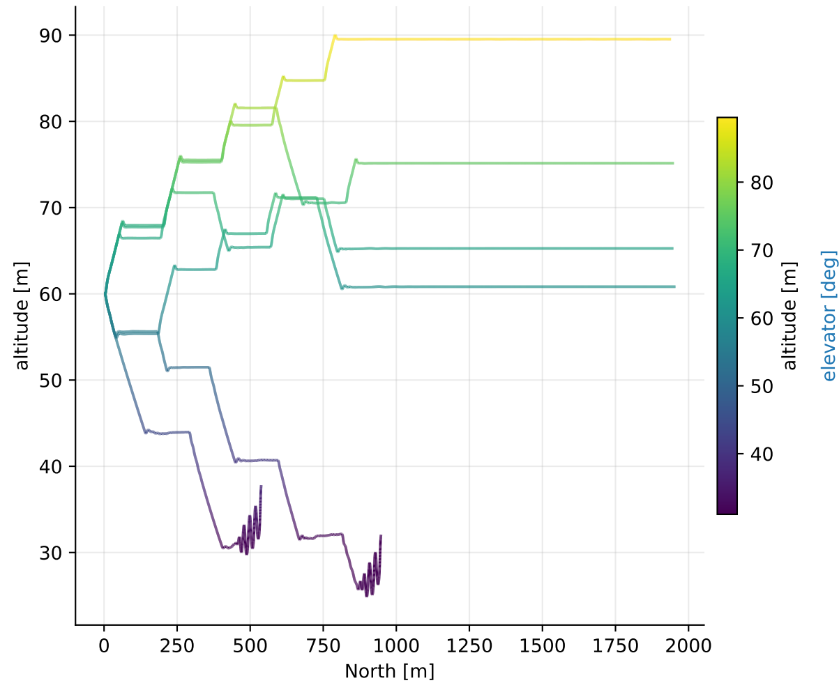
side view (colour = altitude [m])
