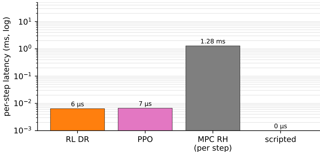
Inference cost (Intel i5-14600K, one thread, JAX CPU, warm JIT)
