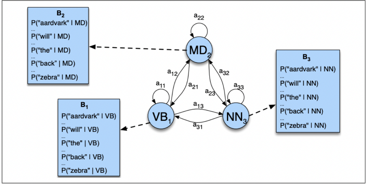
Figure 4.1: An illustration of an HMM for part-of-speech tagging; modelling transition probabilities between POS tags and observation likelihoods for words occurring with these tags. Taken from Jurafsky and Martin 2021c, p. 11
