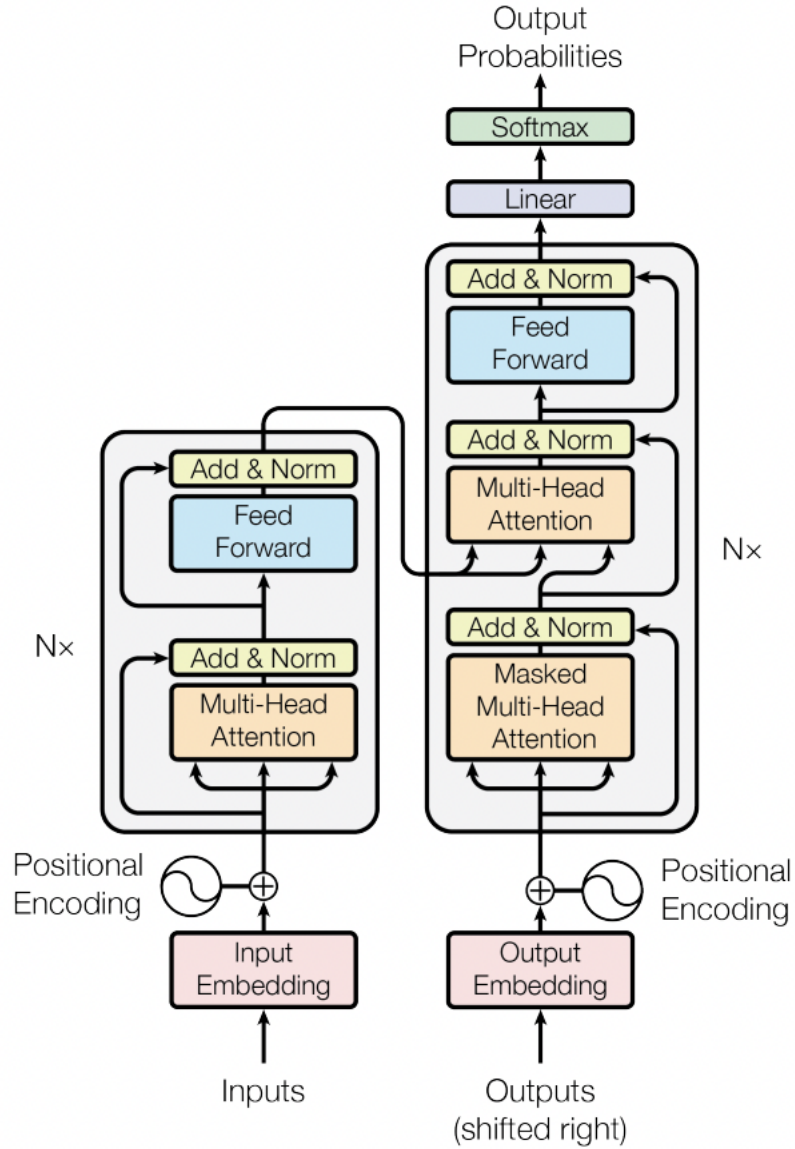
Figure 4.4: Transformer model architecture as introduced by Vaswani et al. 2017
