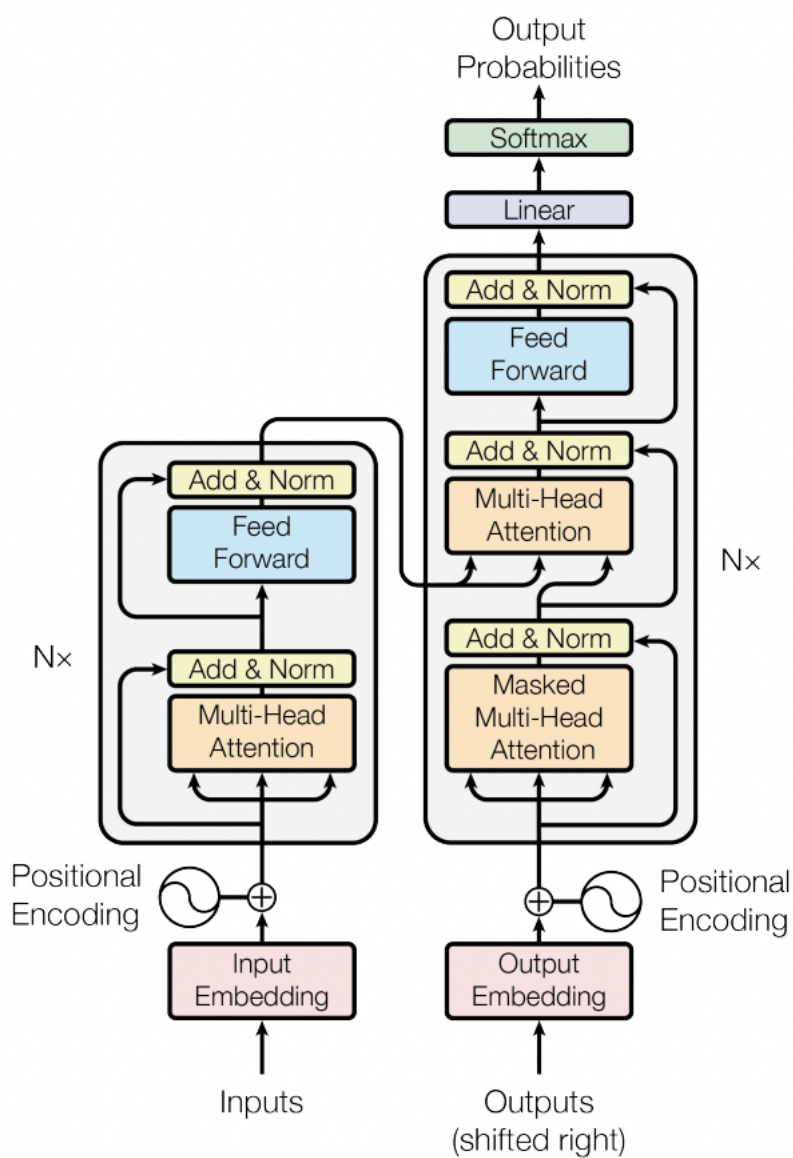
Figure 4.2: Transformer model architecture as introduced by Vaswani et al. 2017
