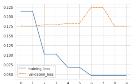
Figure 6.3: Fine-tuning the deepset/gbert-base model: Training and validation loss
