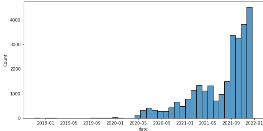
Figure 4.1: Message frequencies
