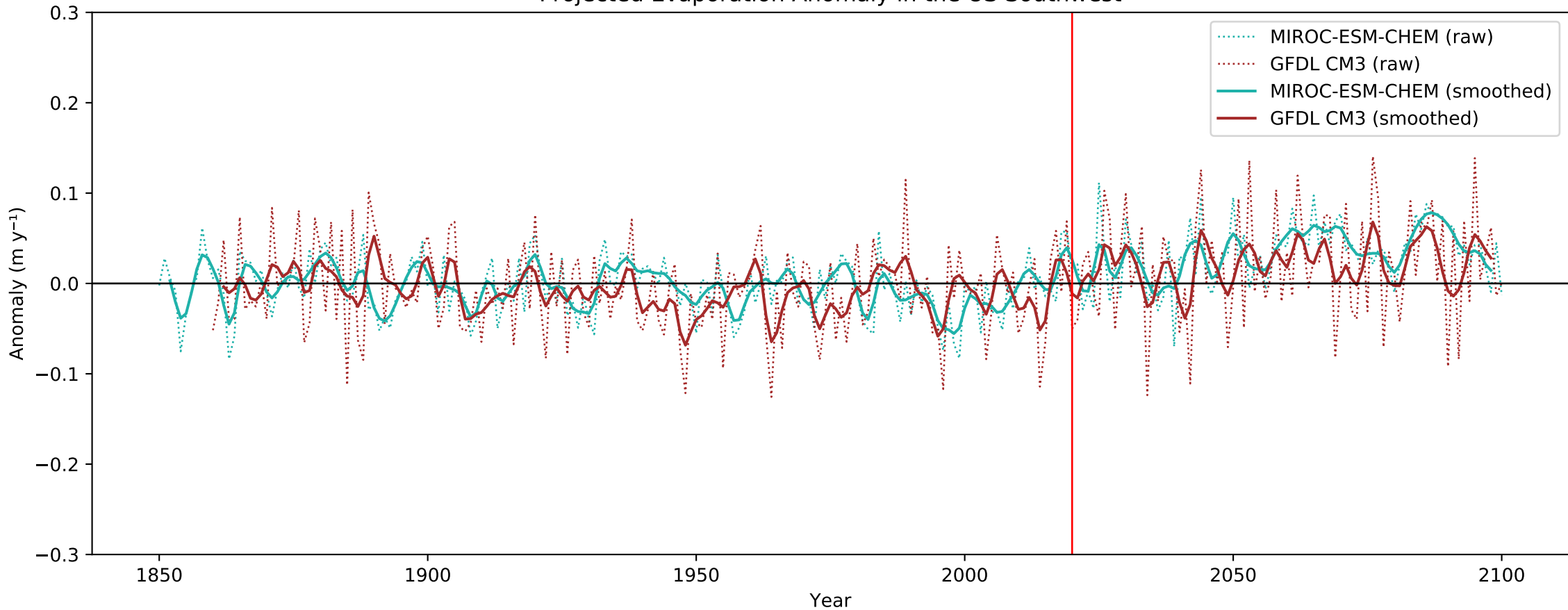
Projected Evaporation Anomaly in the US Southwest
