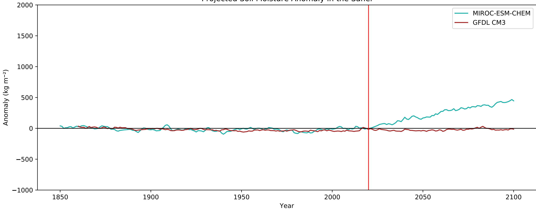
Projected Soil Moisture Anomaly in the Sahel
