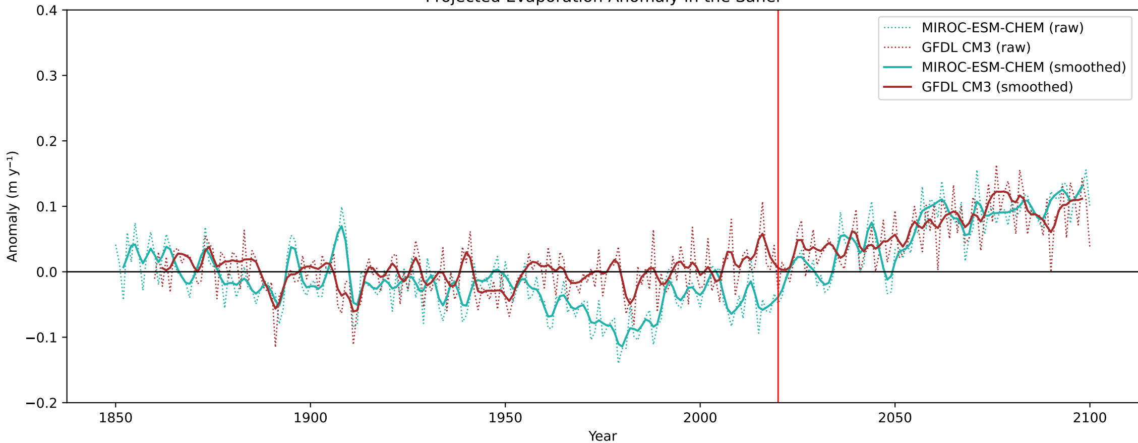
Projected Evaporation Anomaly in the Sahel
