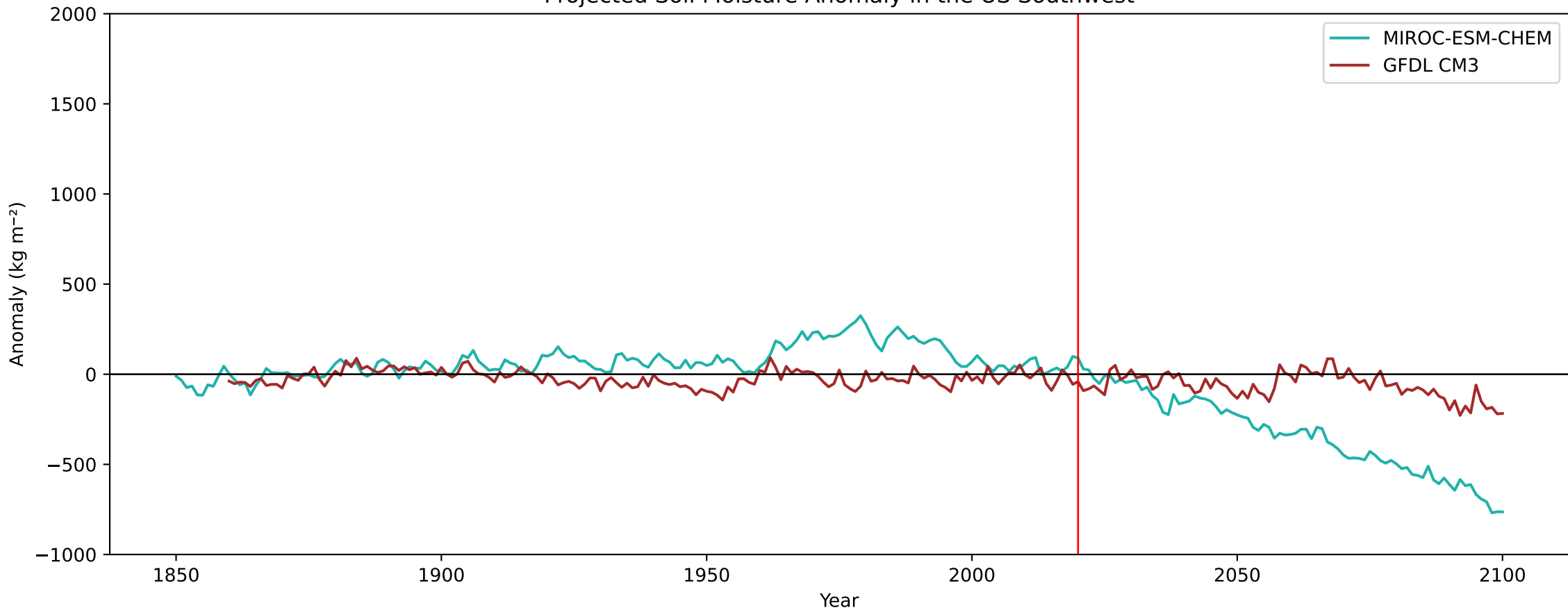
Projected Soil Moisture Anomaly in the US Southwest
