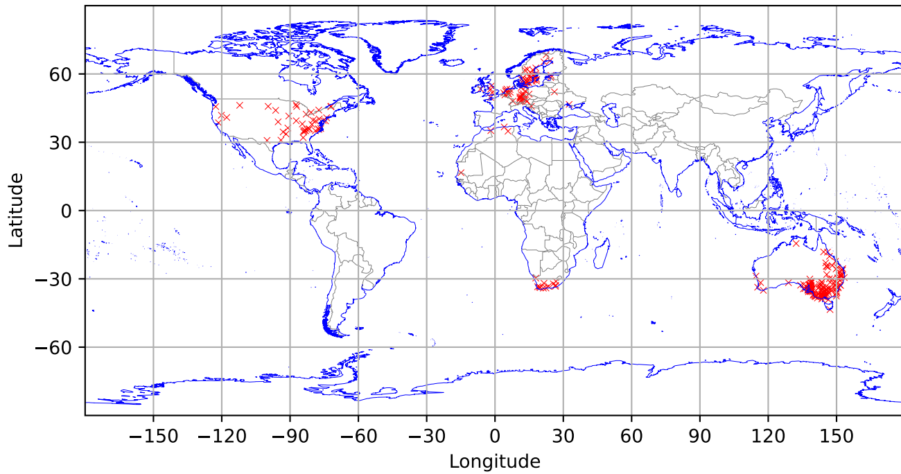
Locations of 275 long-duration stations from 1880 to 2023
