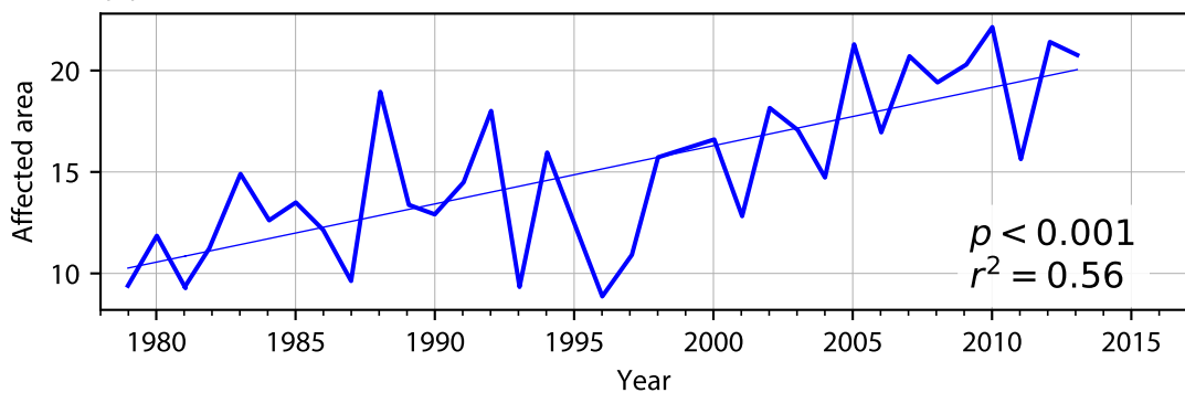
(c) Global fire area
