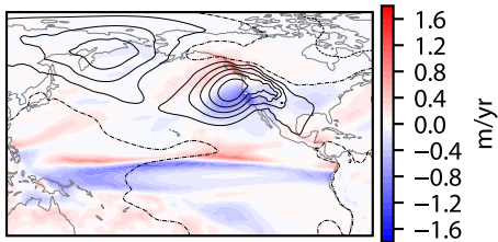
(a) Precipitation, sea-level pressure
