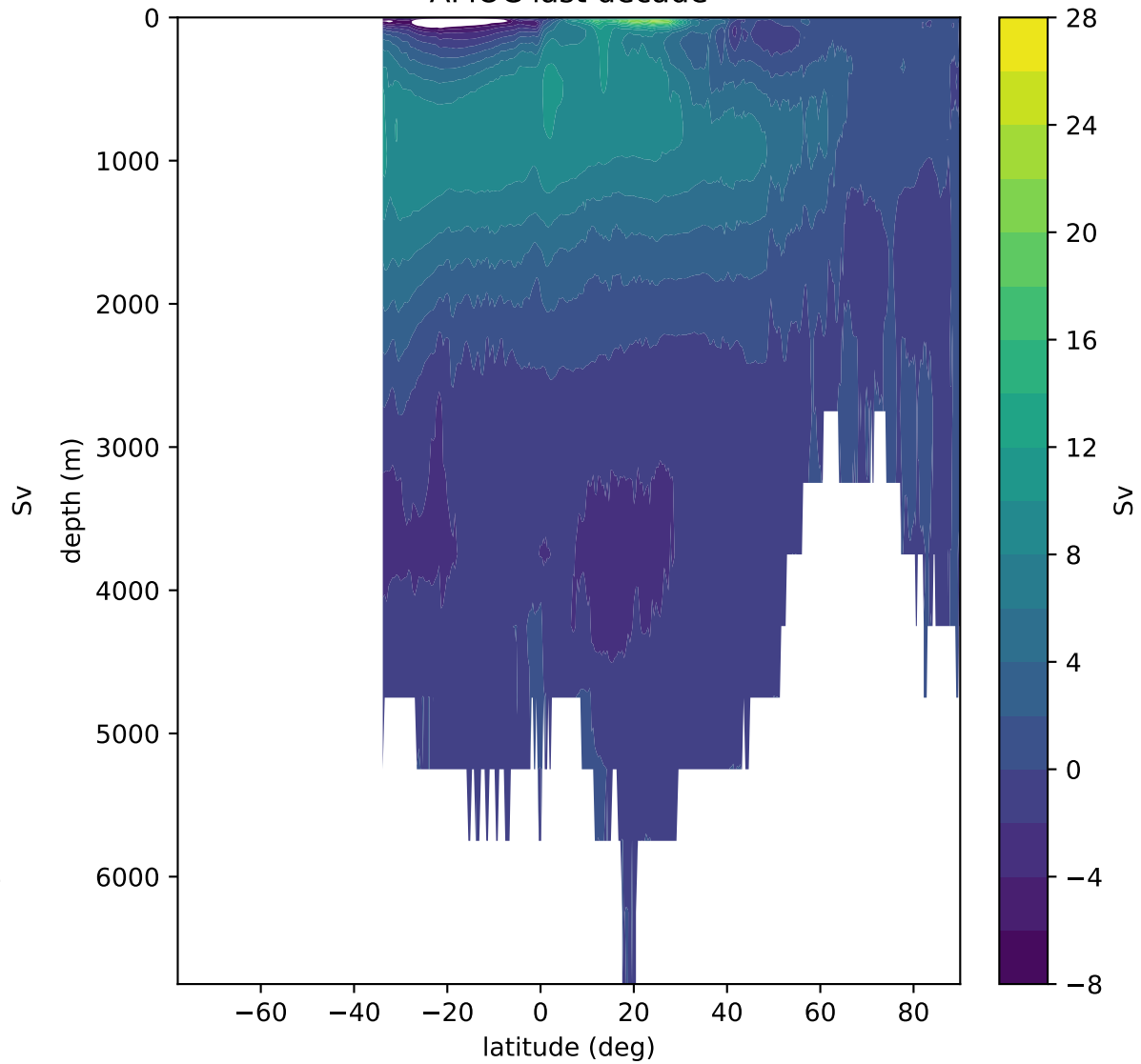
AMOC last decade
