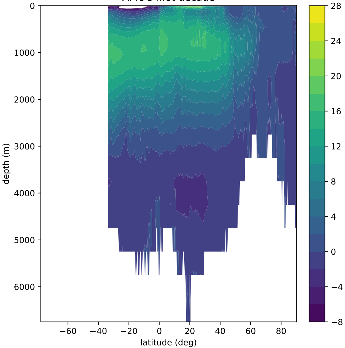
AMOC first decade
