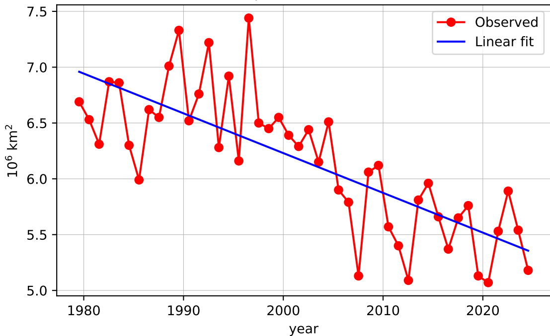
Arctic September sea ice area
