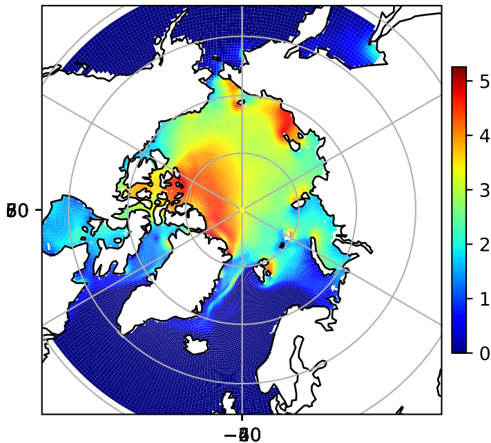
sea ice sic_thickness_obs 1979
