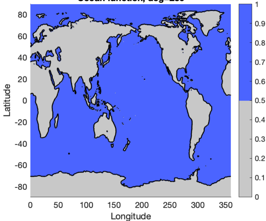
Ocean function, deg=256
