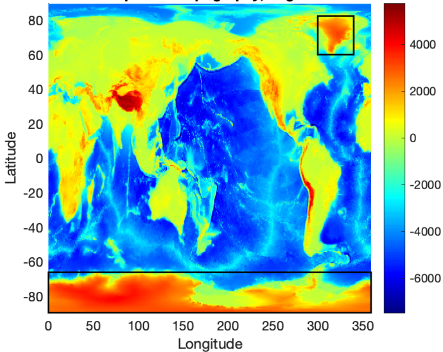
Interpolated topography, deg=256
