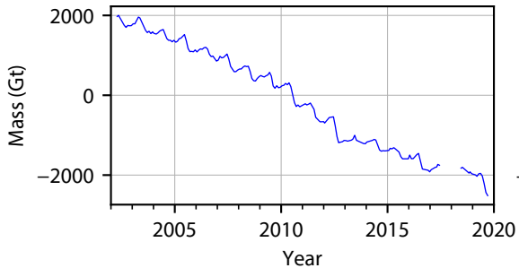
(a) Greenland
