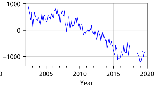
(b) Antarctica
