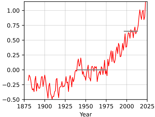
(b) The instrumental record
