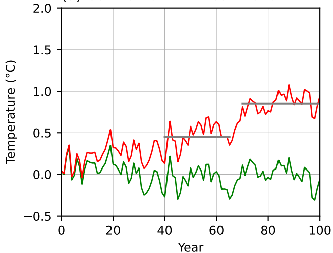
(a) Control run + Linear trend
