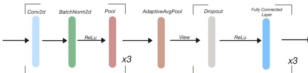
Figure 1: The SimpleNet architecture
