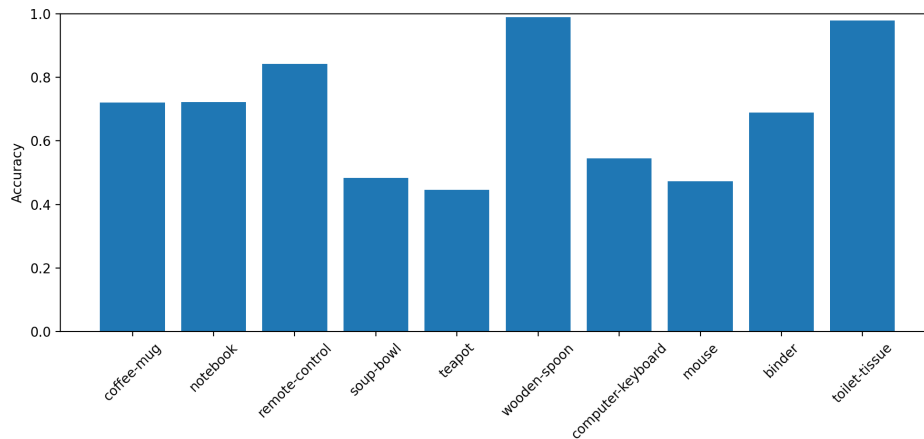
Figure 3: Per-class classification accuracy for ResNet18 without data augmentation on the outdoor test dataset.
