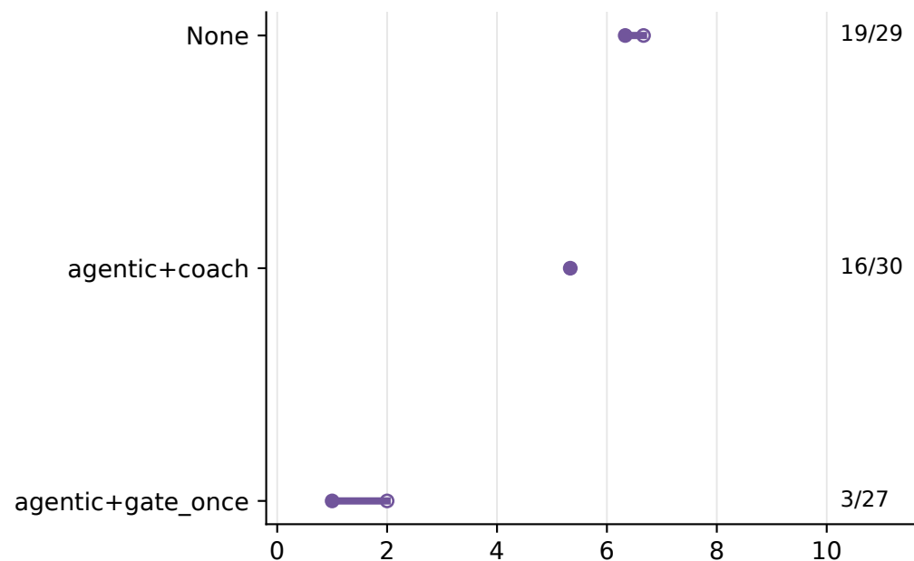
Issue-check counts
