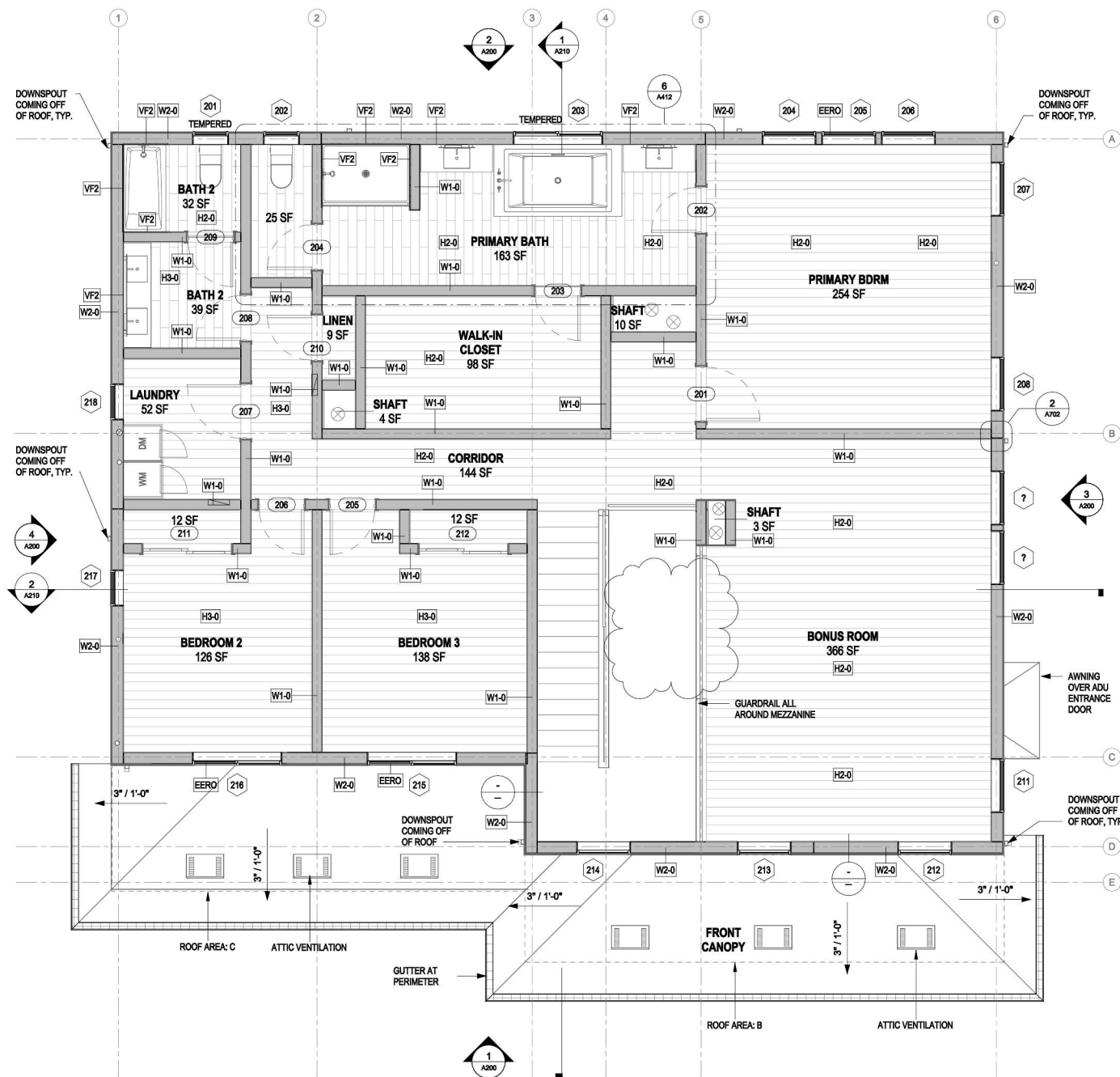
1 FLOOR PLAN - SECOND FLOOR 1/4" = 1'-0"
