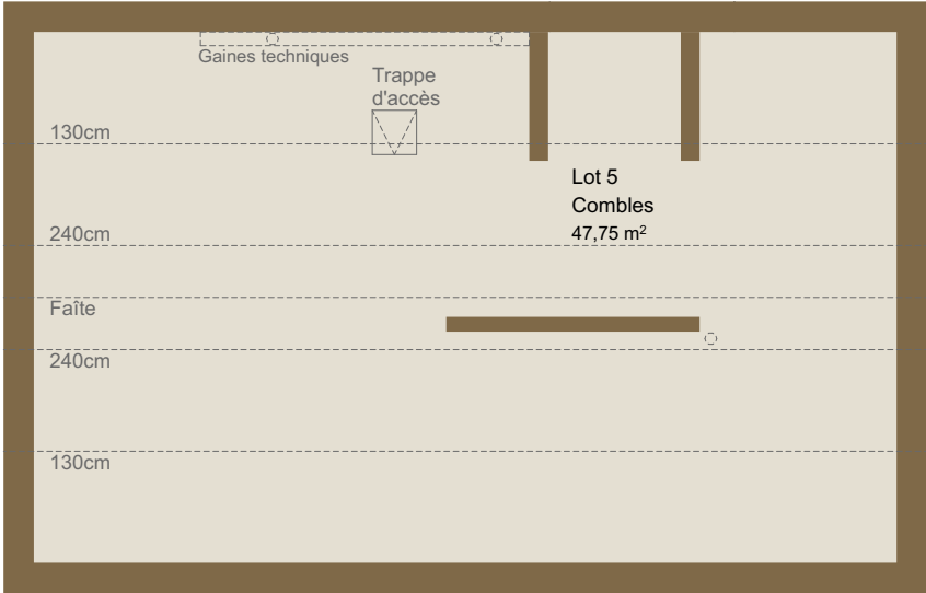
Plan combles
