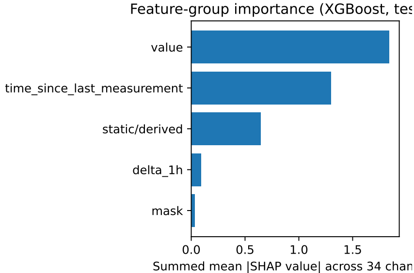
Figure 3: Summed mean |SHAP value| per input-channel group (34 raw clinical variables each), XGBoost baseline, internal test split.
