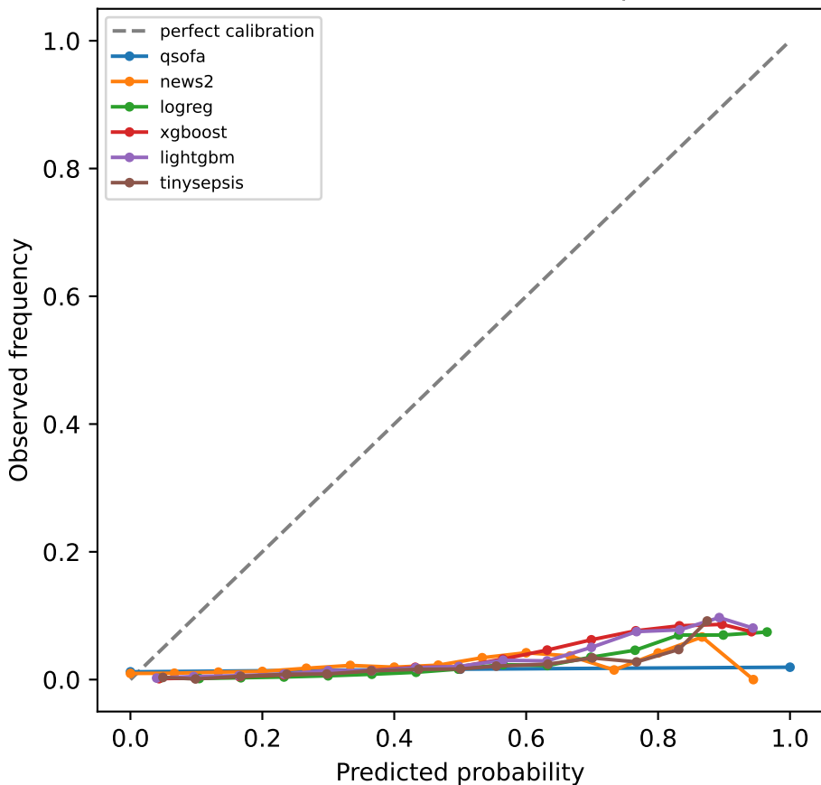
Calibration (test, internal hospital A)
