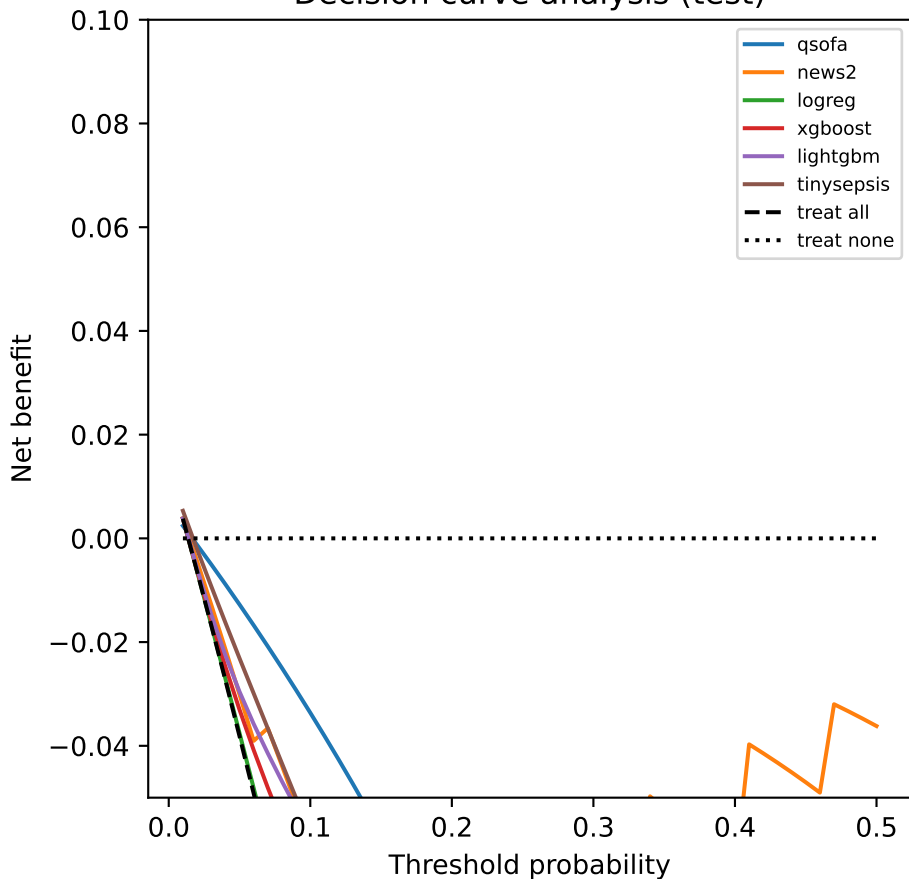
Decision curve analysis (test)
