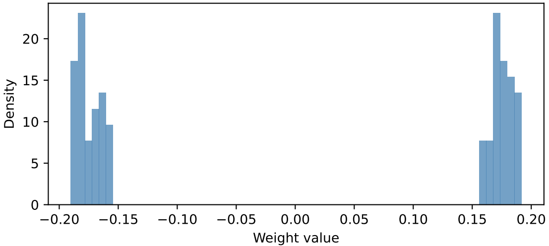
weight Pruned + Quantized Model — Weight Distribution weight
