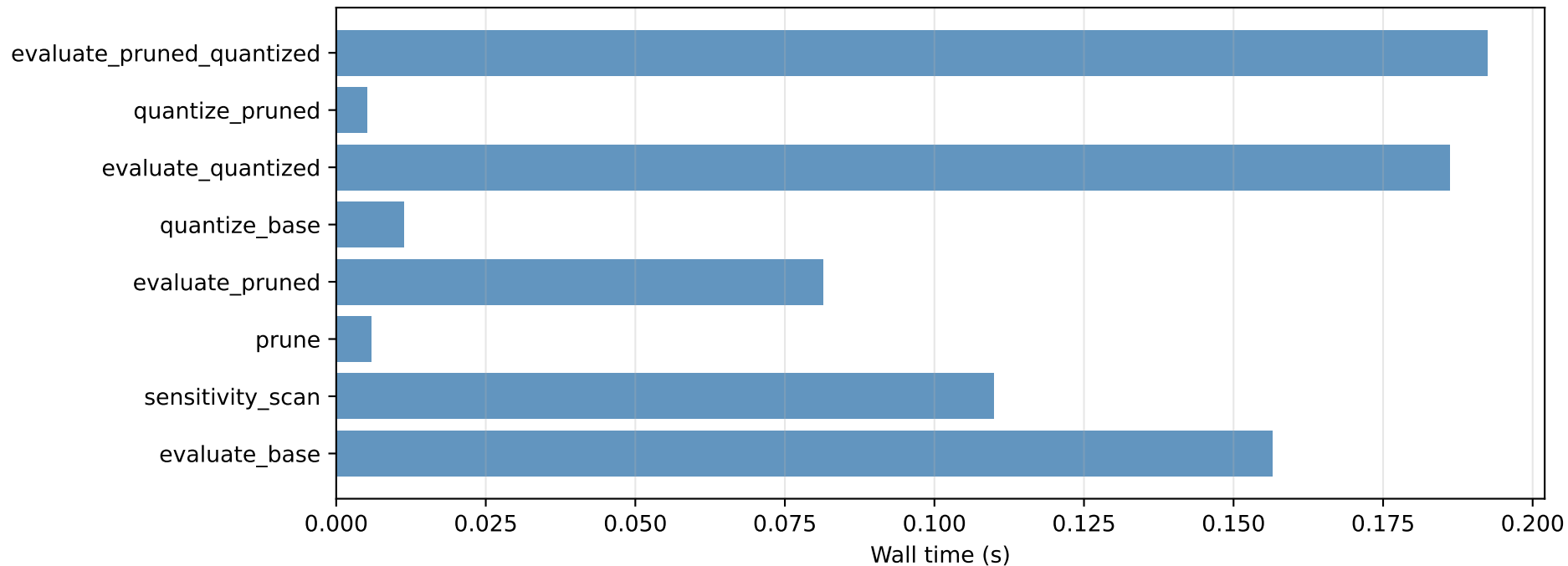
Benchmark — demo-cnn
